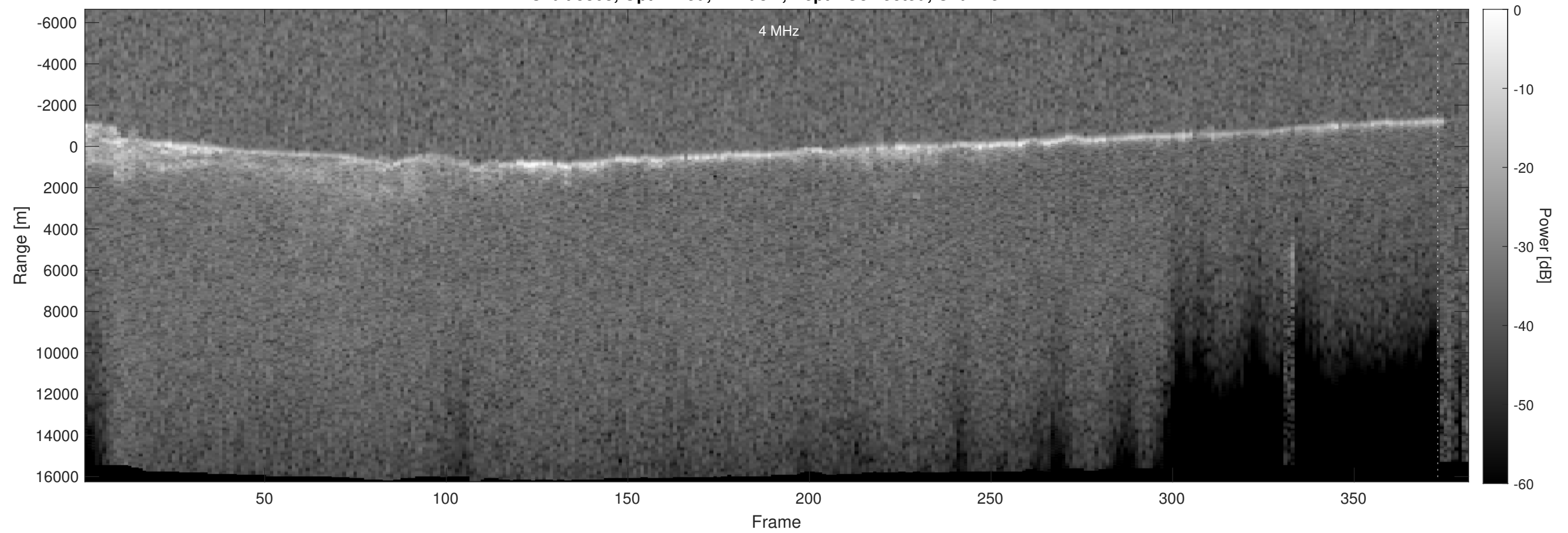
Orbit 5308, Optimized, Window, Depth-Corrected, Channel 2
