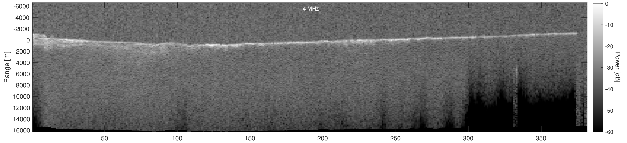
Orbit 5308, Depth-Corrected Cluttergram
