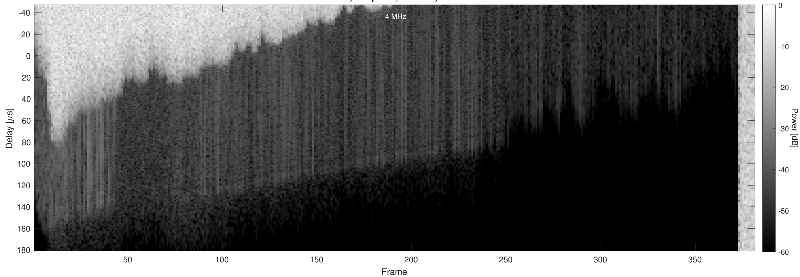
Orbit 5312, Chapman, Window, Channel 2
