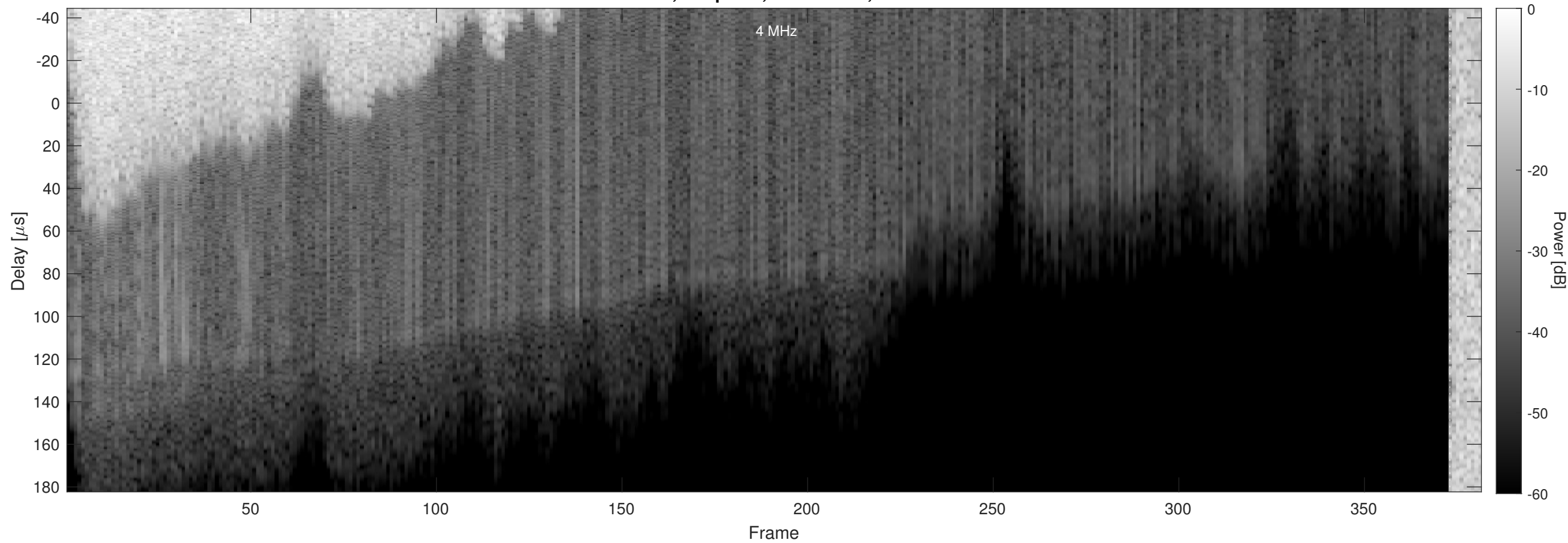
Orbit 5313, Chapman, No Window, Channel 2
