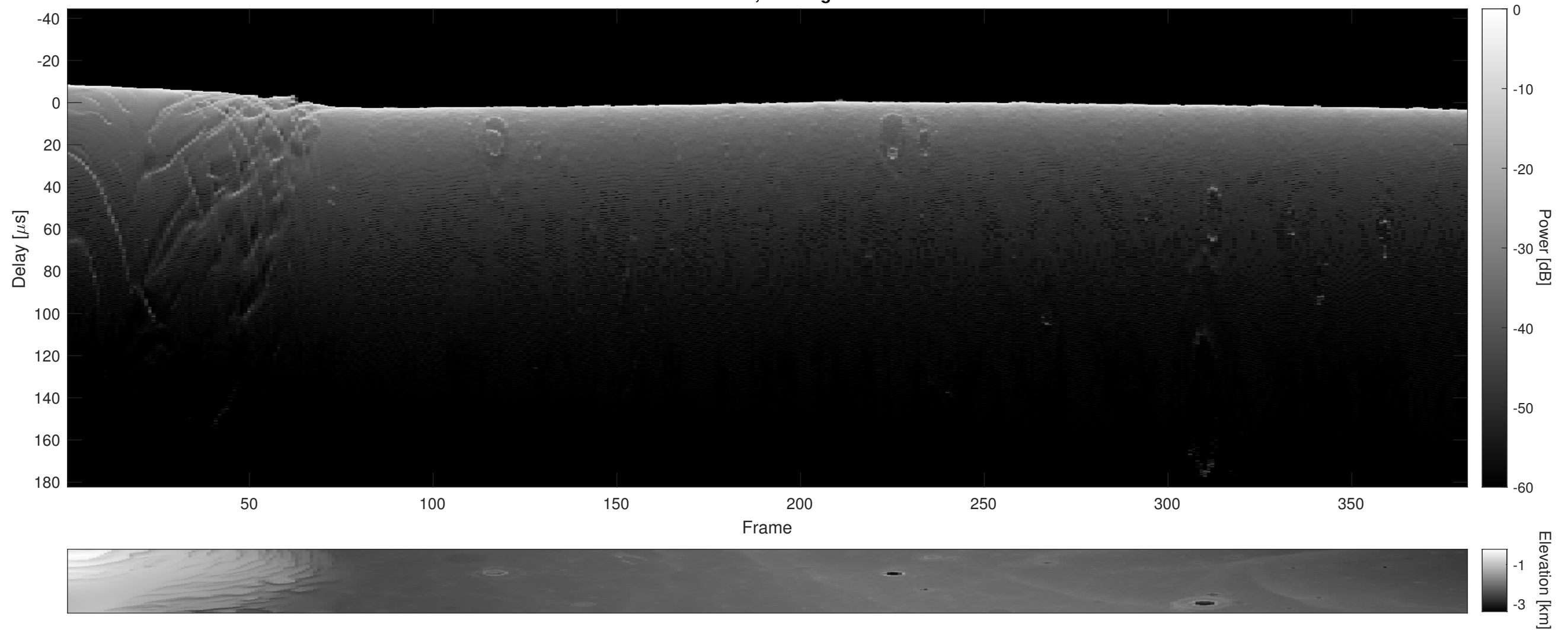
Orbit 5313, Cluttergram
