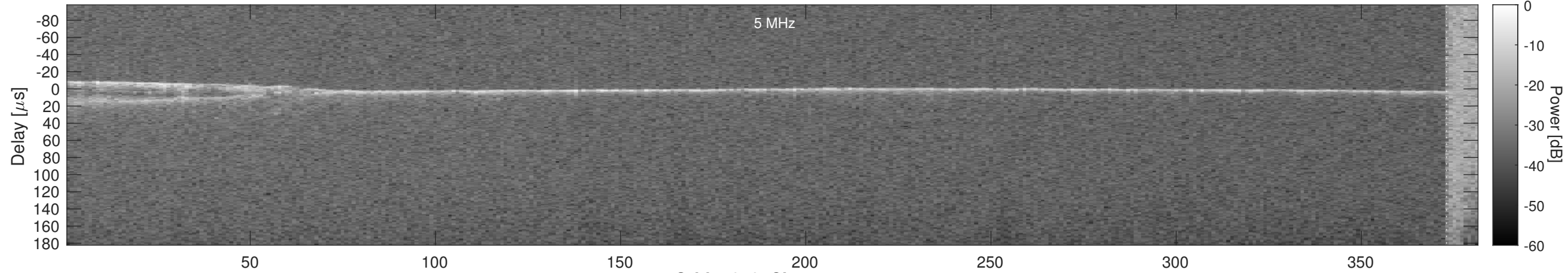
Orbit 5313, Cluttergram
