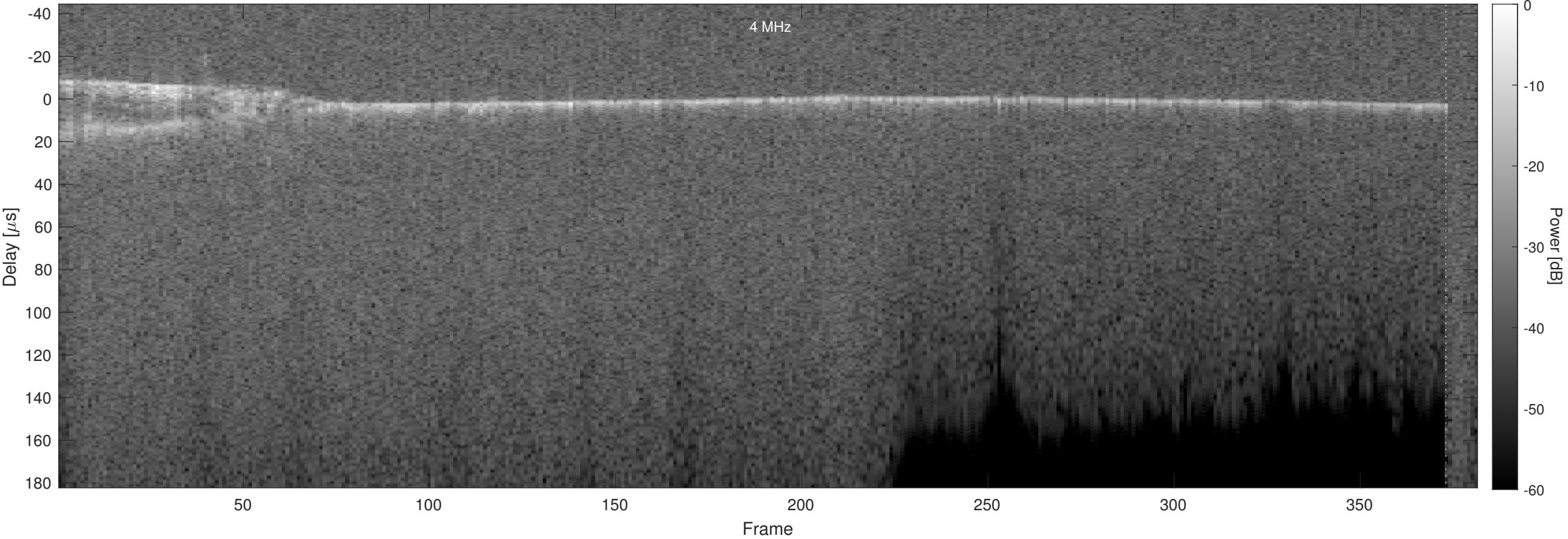
Orbit 5313, Optimized, No Window, Channel 2
