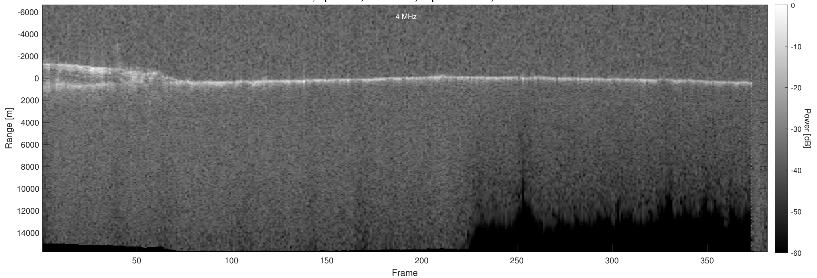
Orbit 5313, Optimized, No Window, Depth-Corrected, Channel 2
