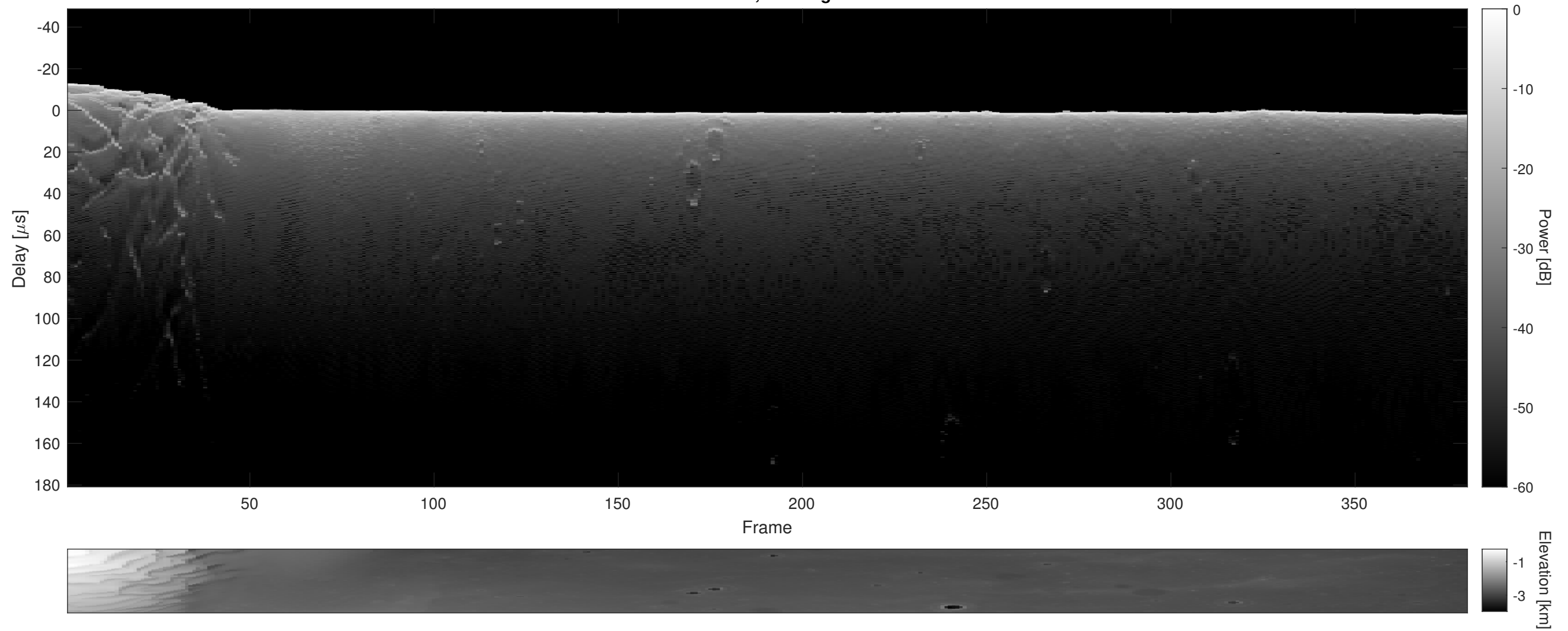
Orbit 5316, Cluttergram
