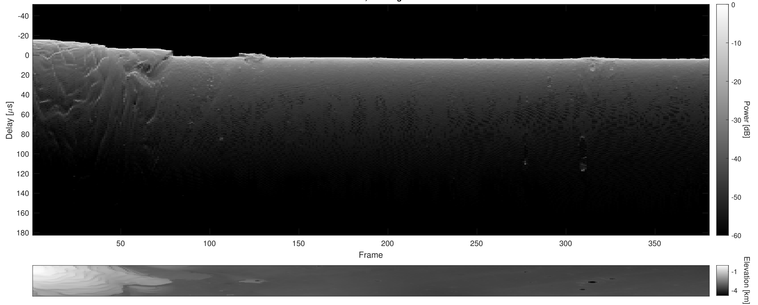
Orbit 5318, Cluttergram
