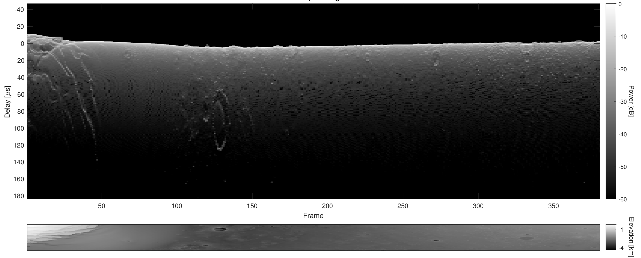
Orbit 5319, Cluttergram
