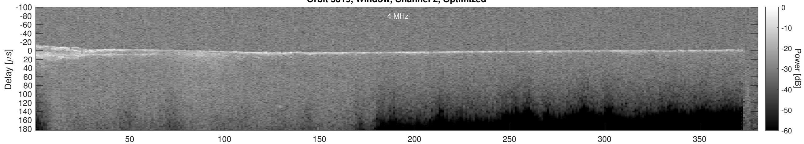
Orbit 5319, Cluttergram
