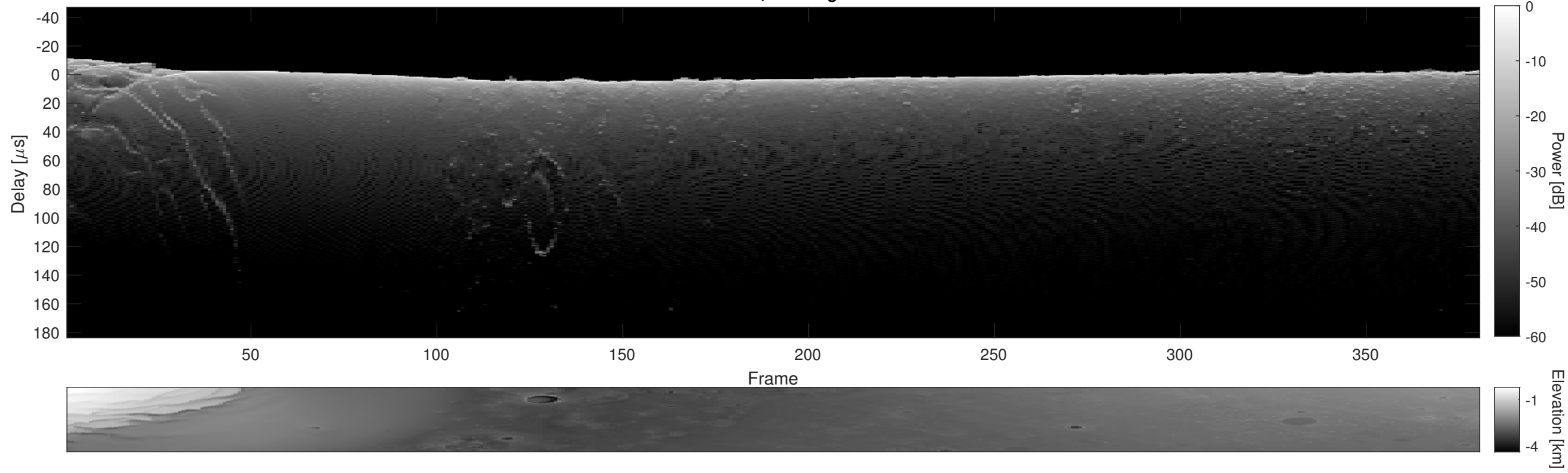
Orbit 5319, Cluttergram
