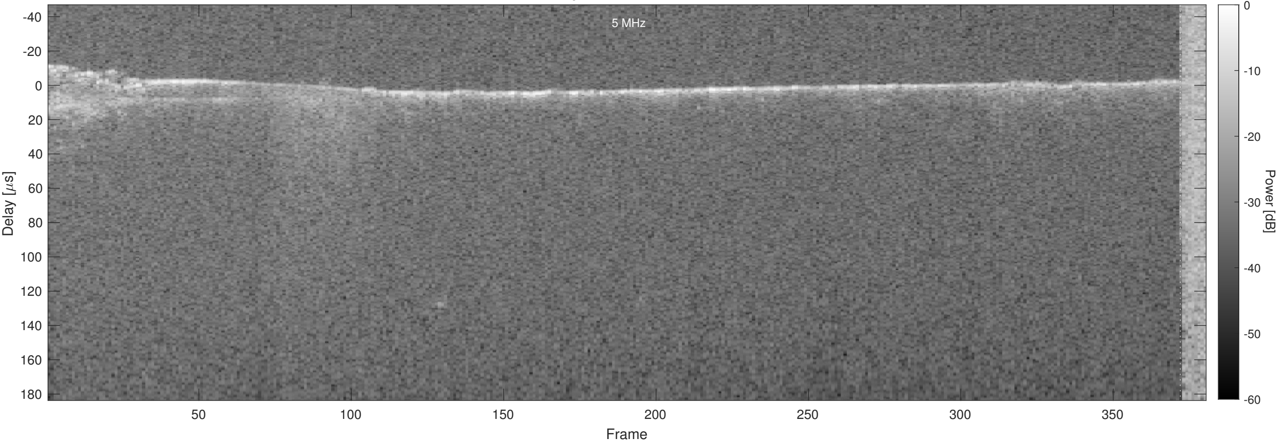
Orbit 5319, Optimized, Window, Channel 2
