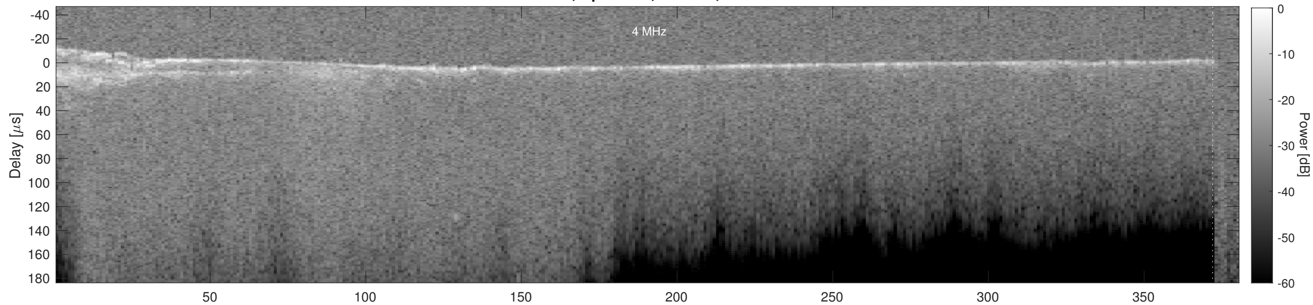
Orbit 5319, Cluttergram
