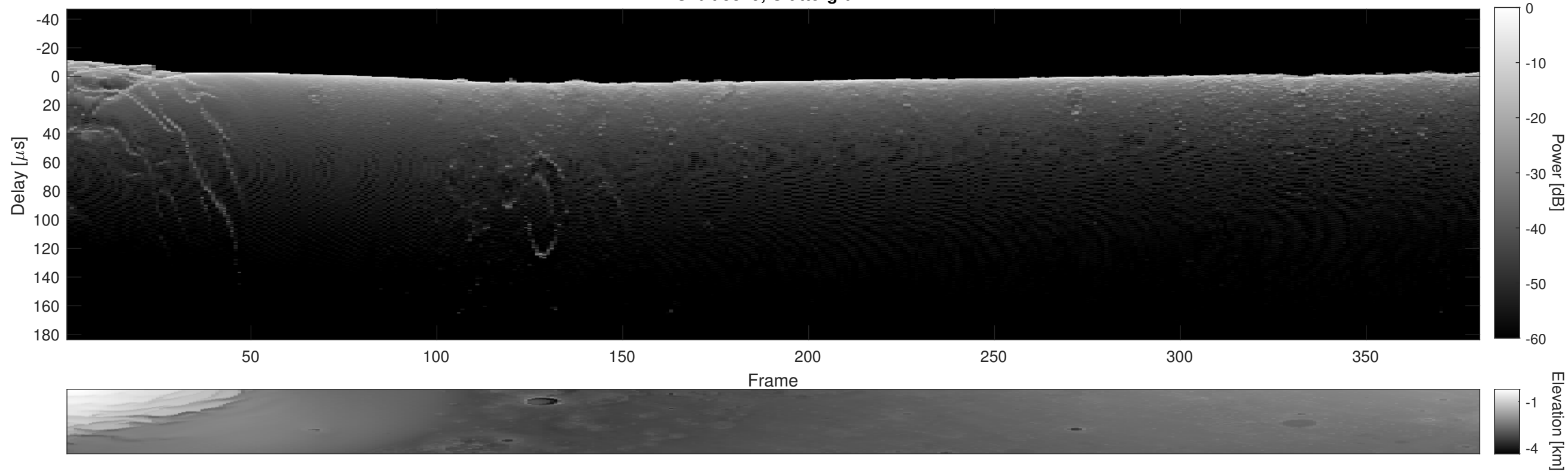
Orbit 5319, Cluttergram
