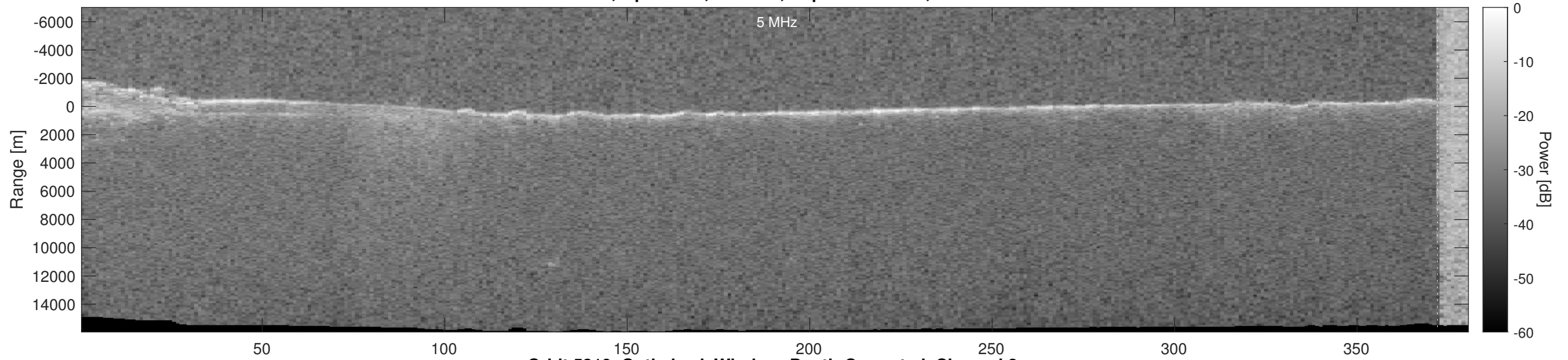
Orbit 5319, Optimized, Window, Depth-Corrected, Channel 2
