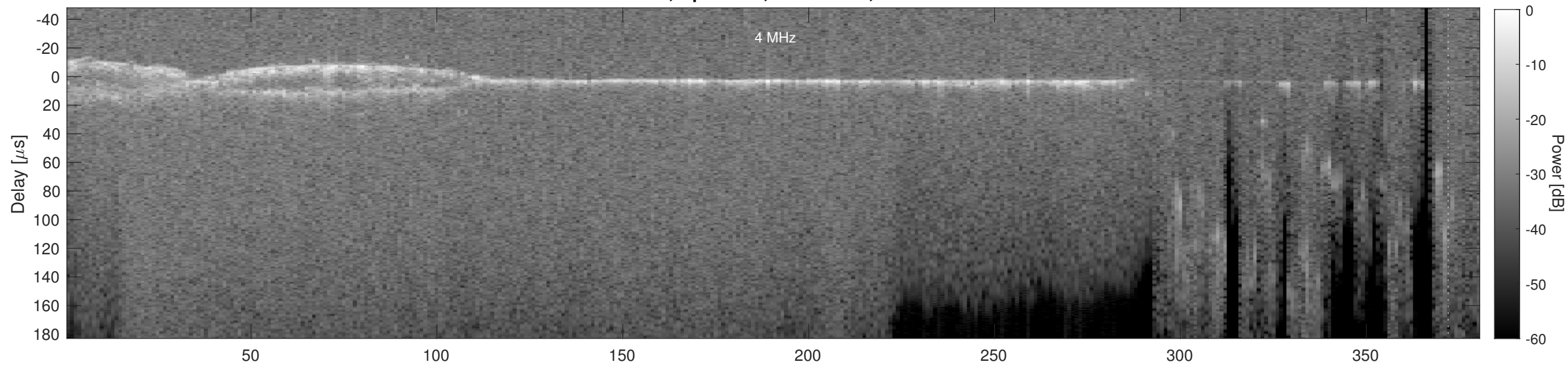
Orbit 5321, Cluttergram
