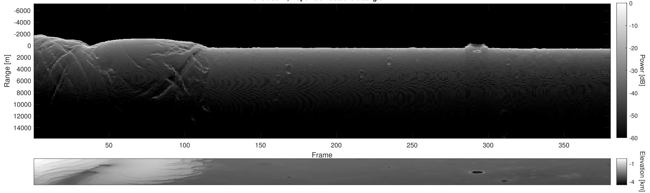
Orbit 5321, Depth-Corrected Cluttergram
