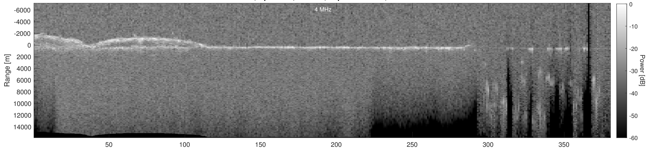
Orbit 5321, Depth-Corrected Cluttergram
