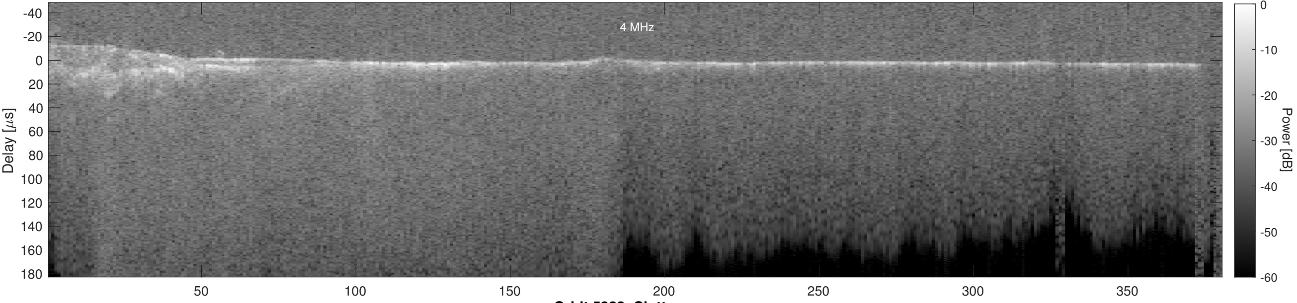
Orbit 5323, Cluttergram
