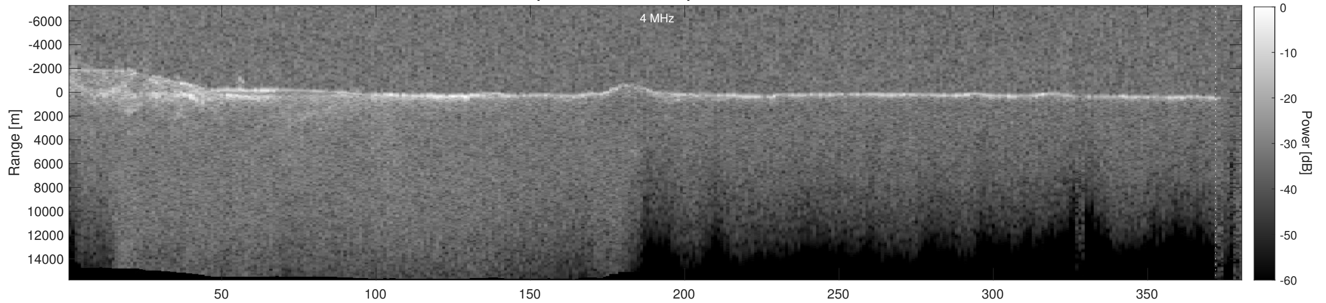
Orbit 5323, Depth-Corrected Cluttergram
