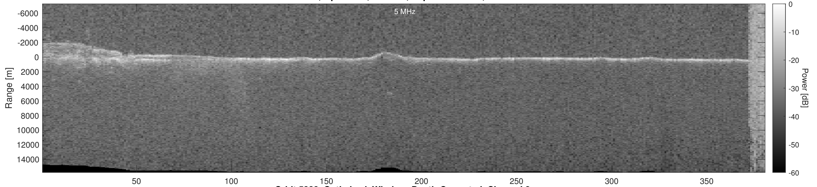
Orbit 5323, Optimized, Window, Depth-Corrected, Channel 2
