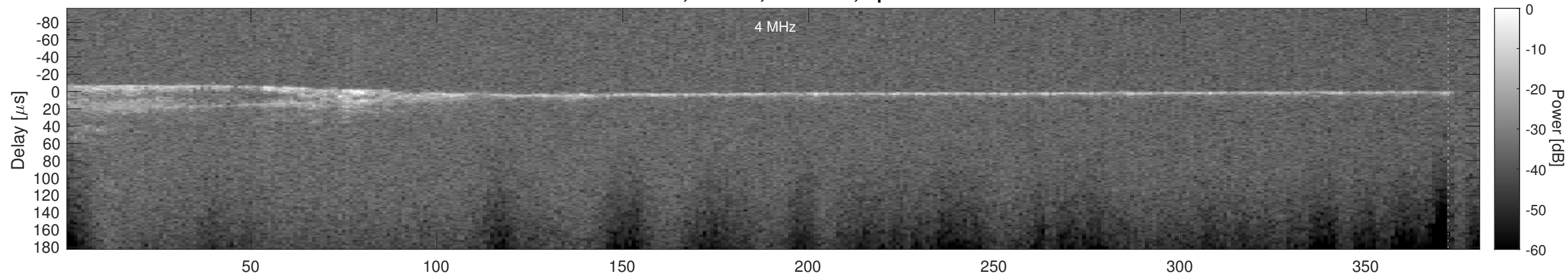
Orbit 5324, Cluttergram
