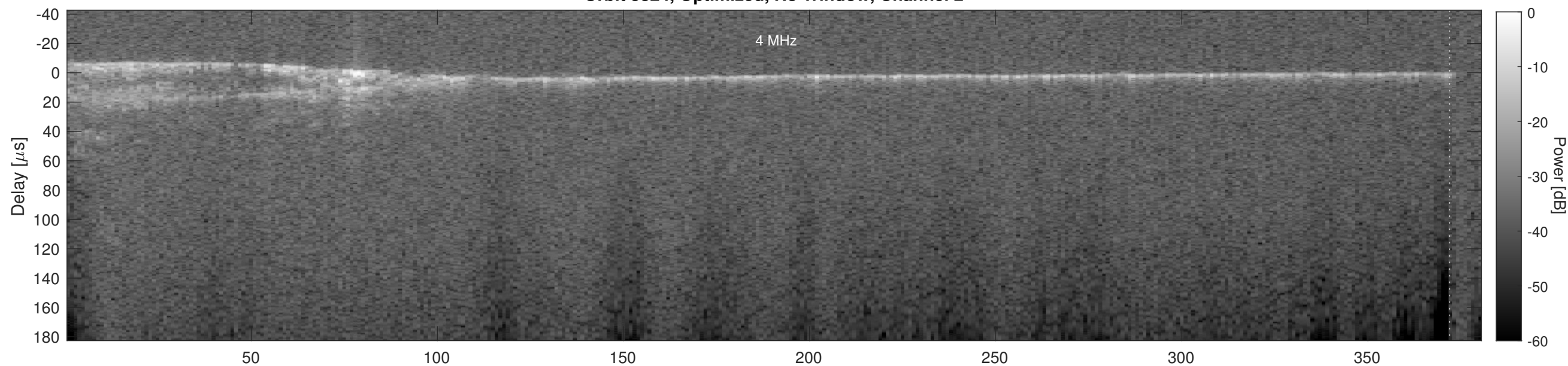
Orbit 5324, Cluttergram
