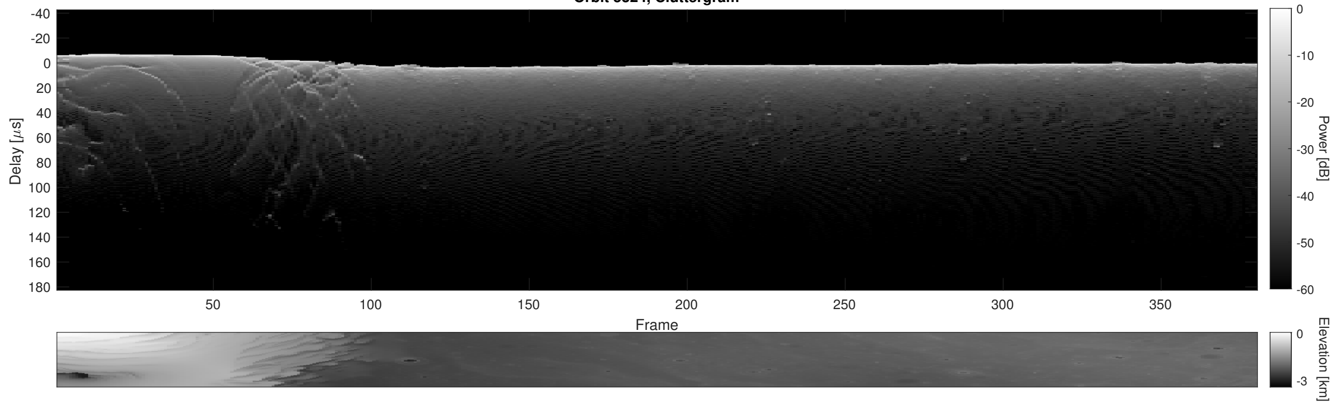
Orbit 5324, Cluttergram
