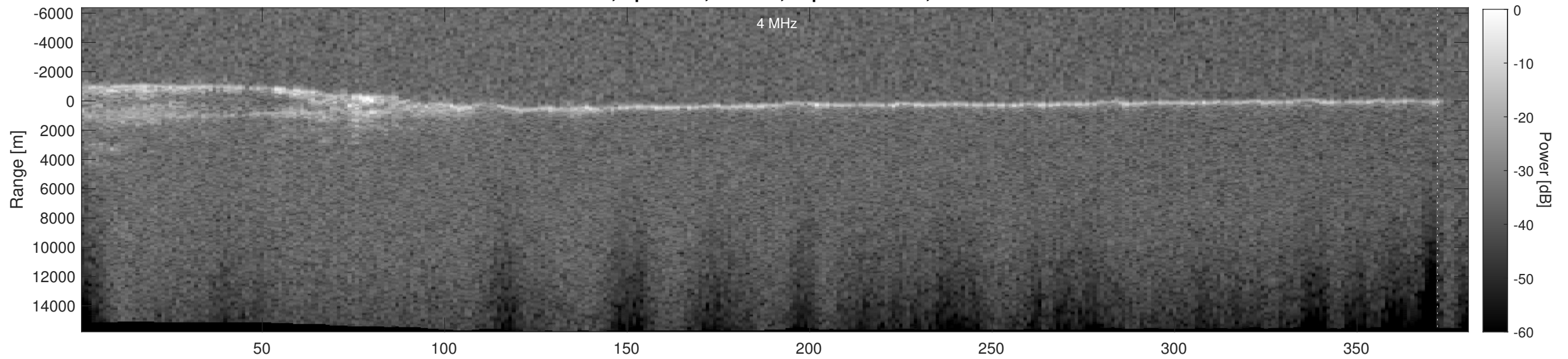
Orbit 5324, Depth-Corrected Cluttergram
