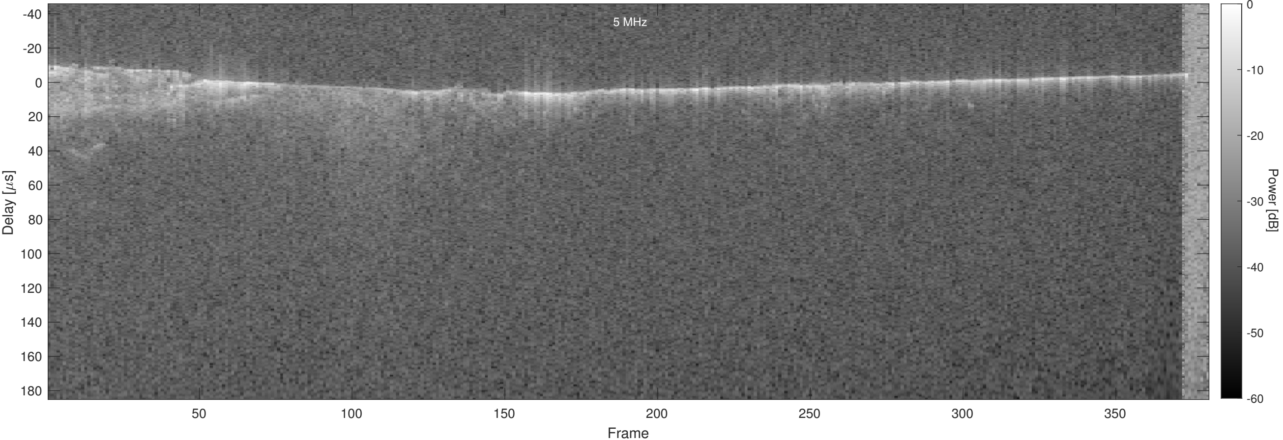
Orbit 5326, Optimized, No Window, Channel 2
