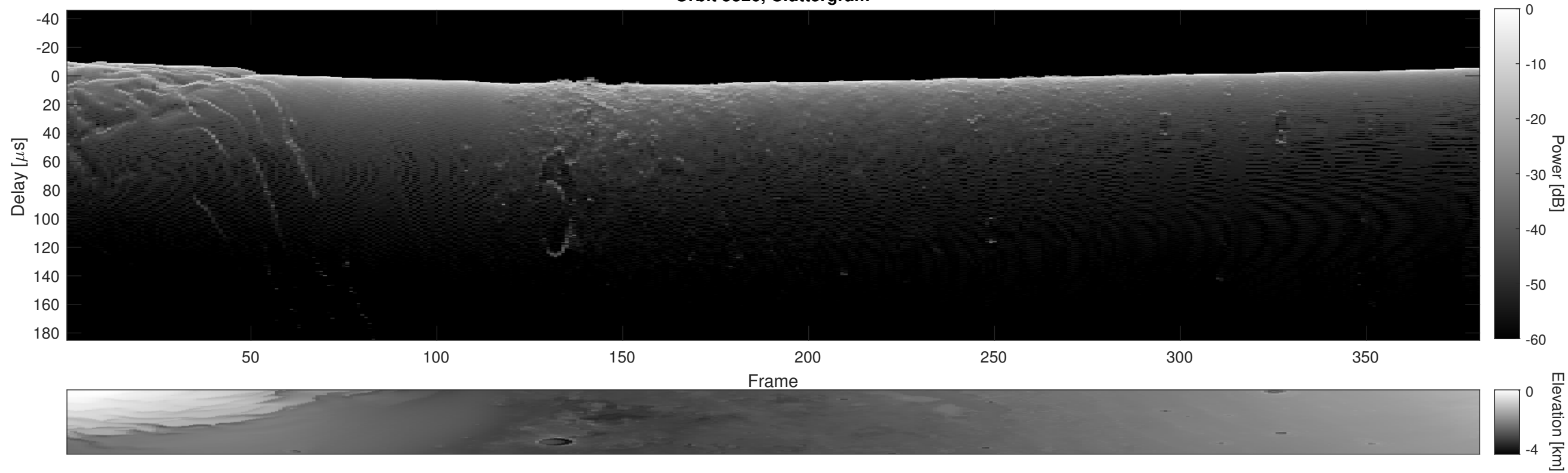
Orbit 5326, Cluttergram
