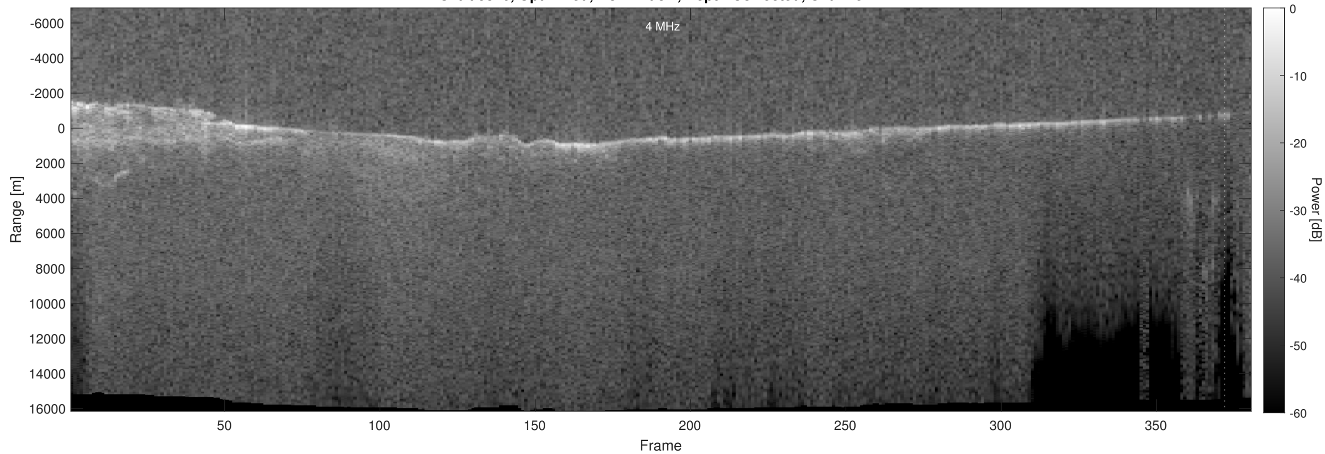
Orbit 5326, Optimized, No Window, Depth-Corrected, Channel 2
