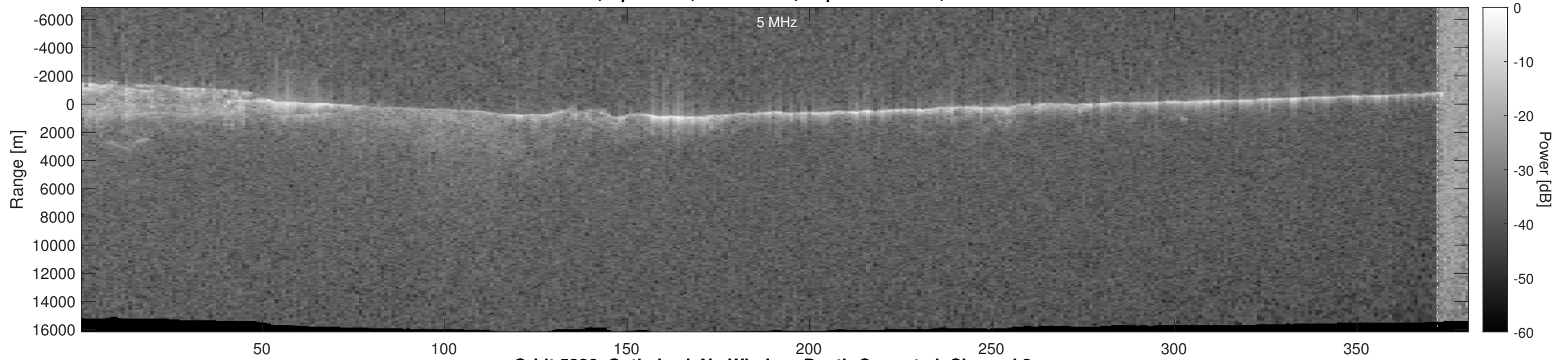
Orbit 5326, Optimized, No Window, Depth-Corrected, Channel 2
