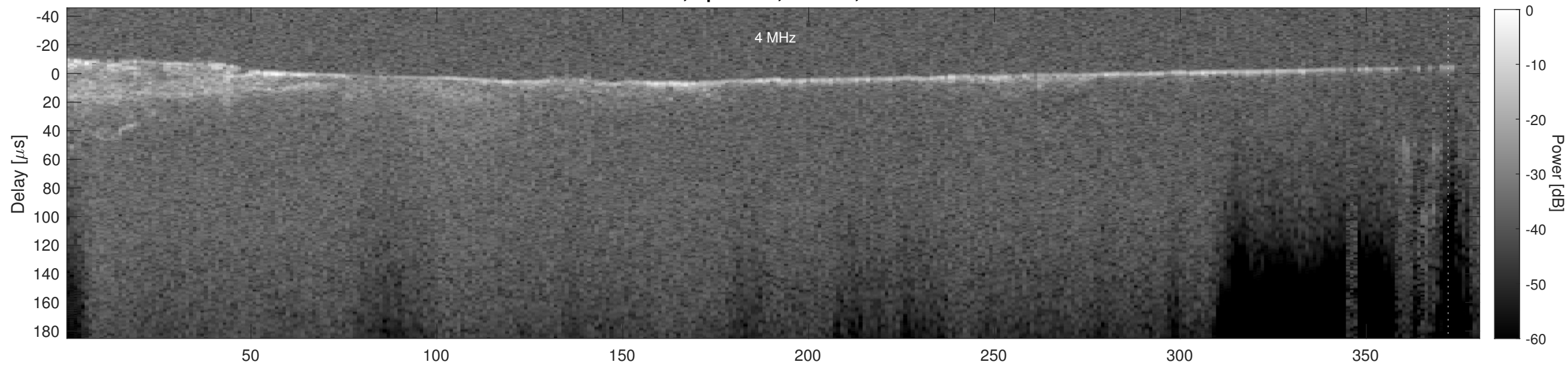
Orbit 5326, Cluttergram
