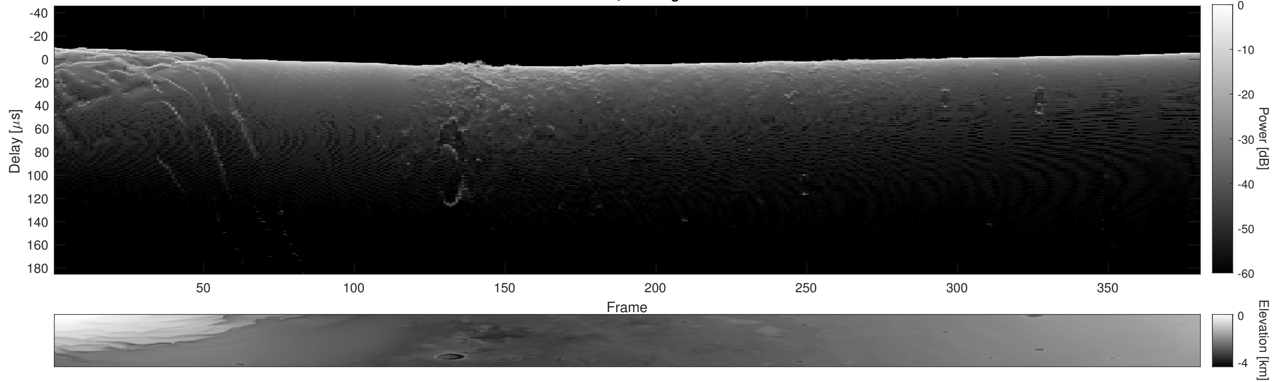
Orbit 5326, Cluttergram
