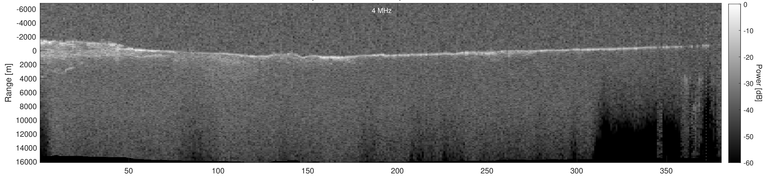
Orbit 5326, Depth-Corrected Cluttergram
