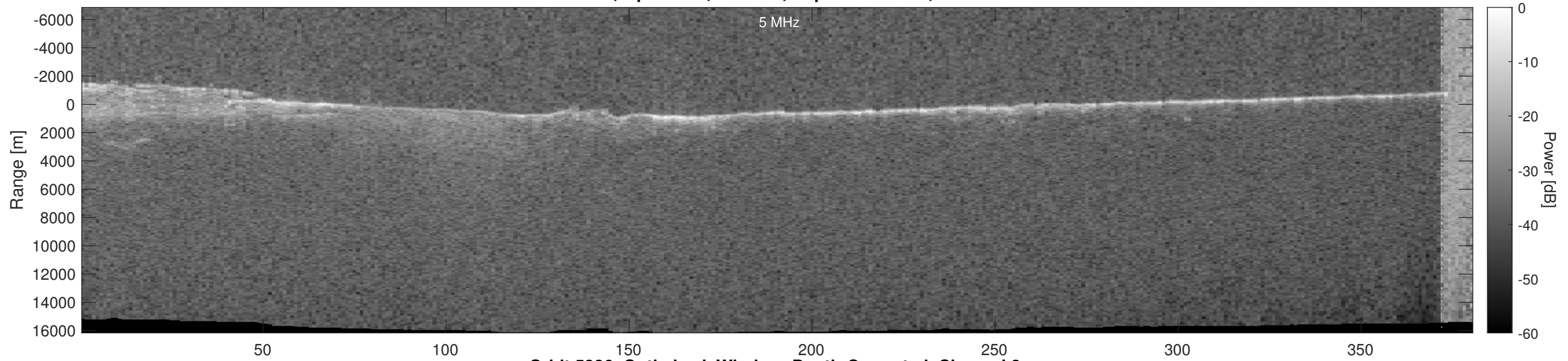
Orbit 5326, Optimized, Window, Depth-Corrected, Channel 2
