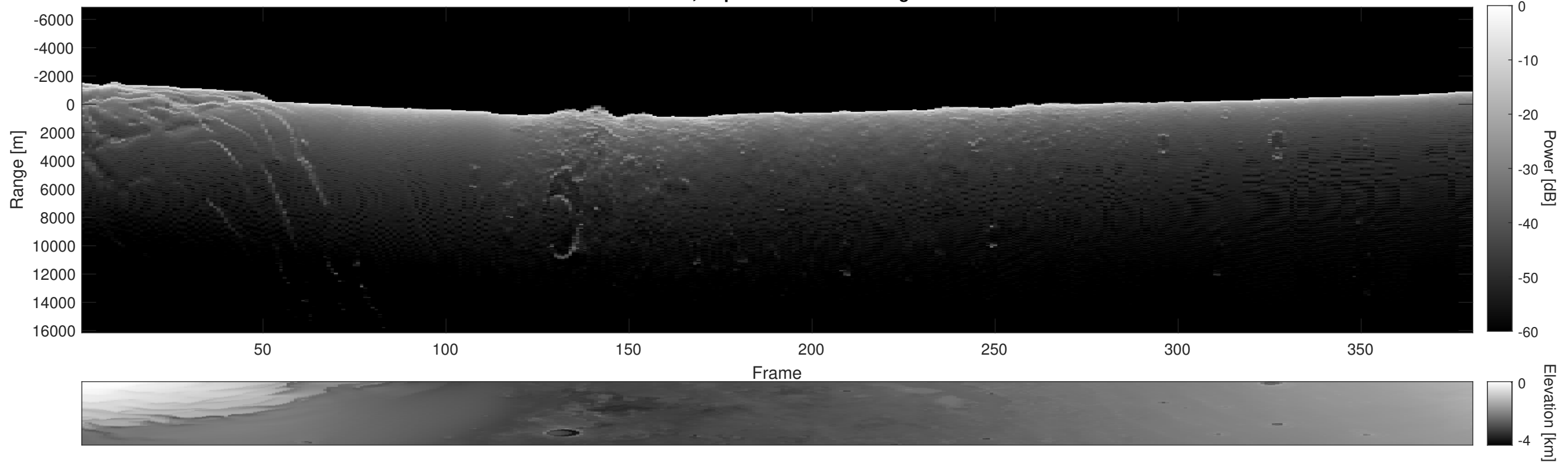
Orbit 5326, Depth-Corrected Cluttergram
