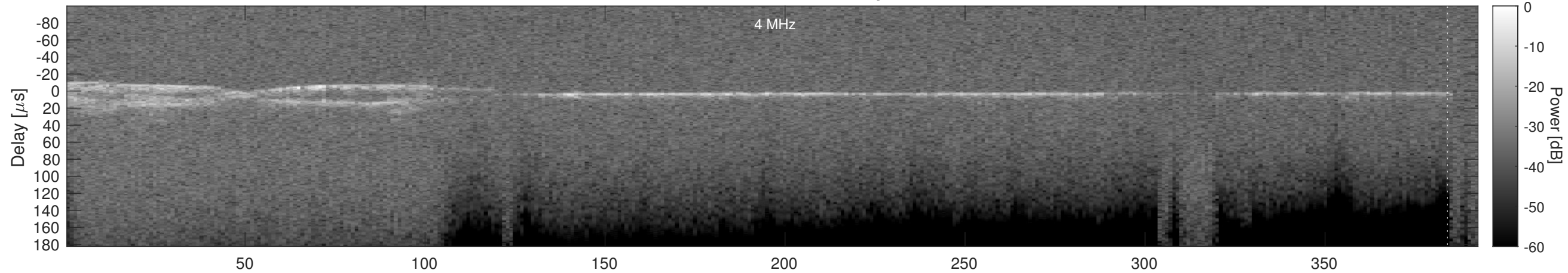
Orbit 5328, Cluttergram
