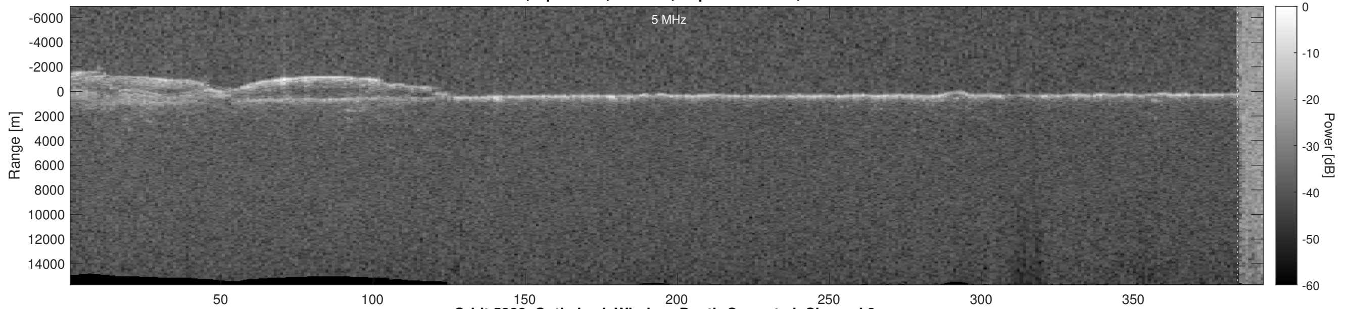
Orbit 5328, Optimized, Window, Depth-Corrected, Channel 2
