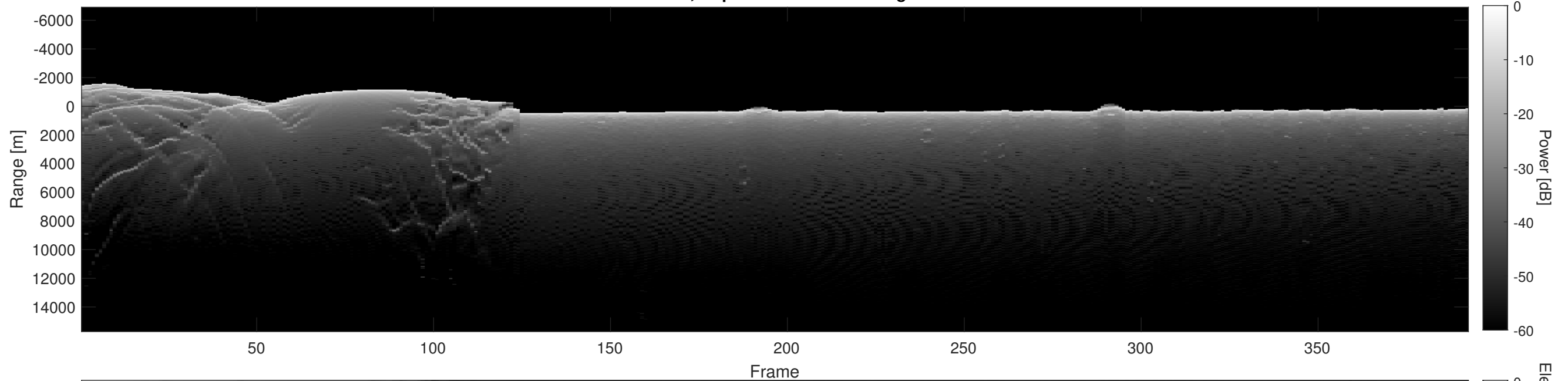
Orbit 5328, Depth-Corrected Cluttergram
