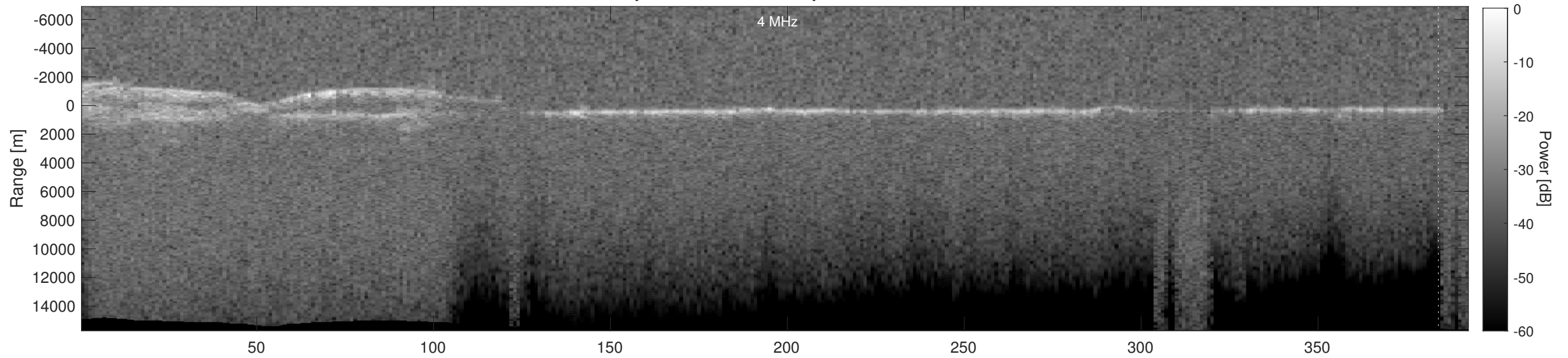
Orbit 5328, Depth-Corrected Cluttergram
