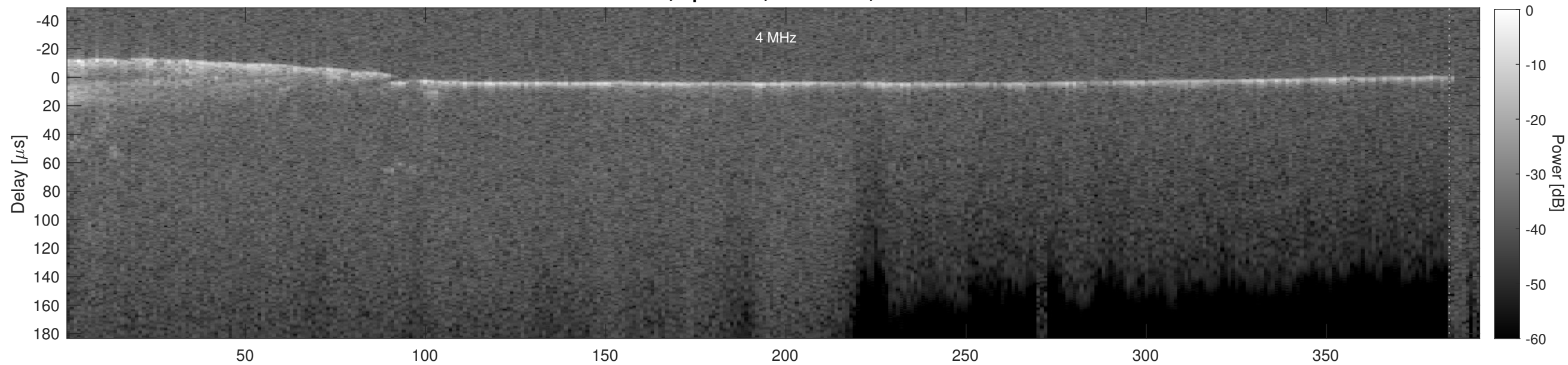
Orbit 5329, Cluttergram
