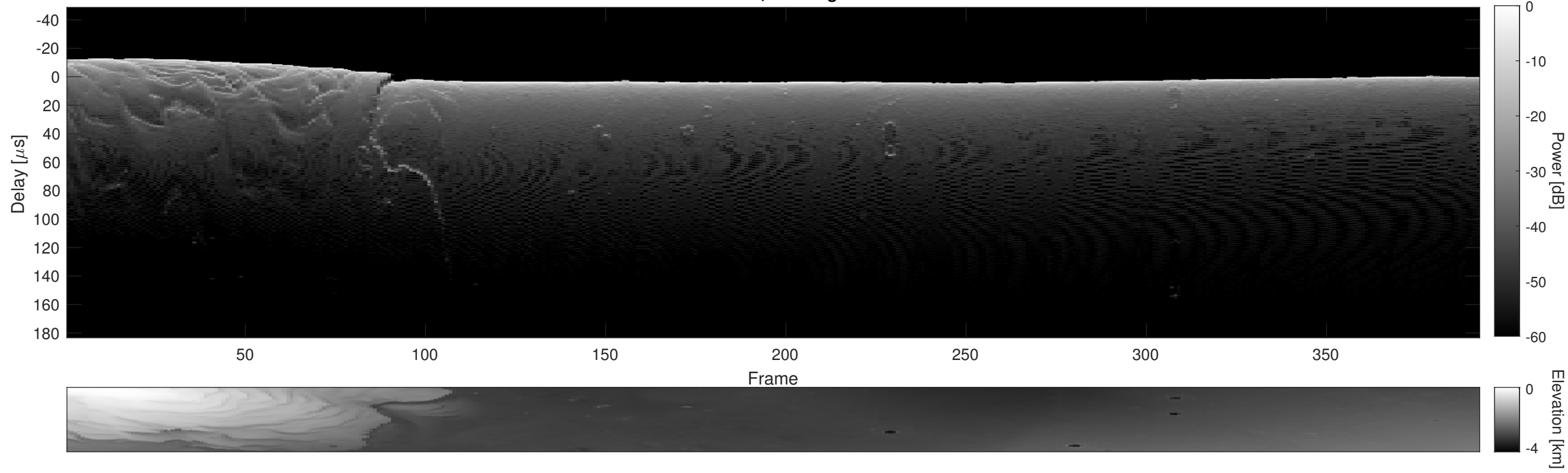
Orbit 5329, Cluttergram
