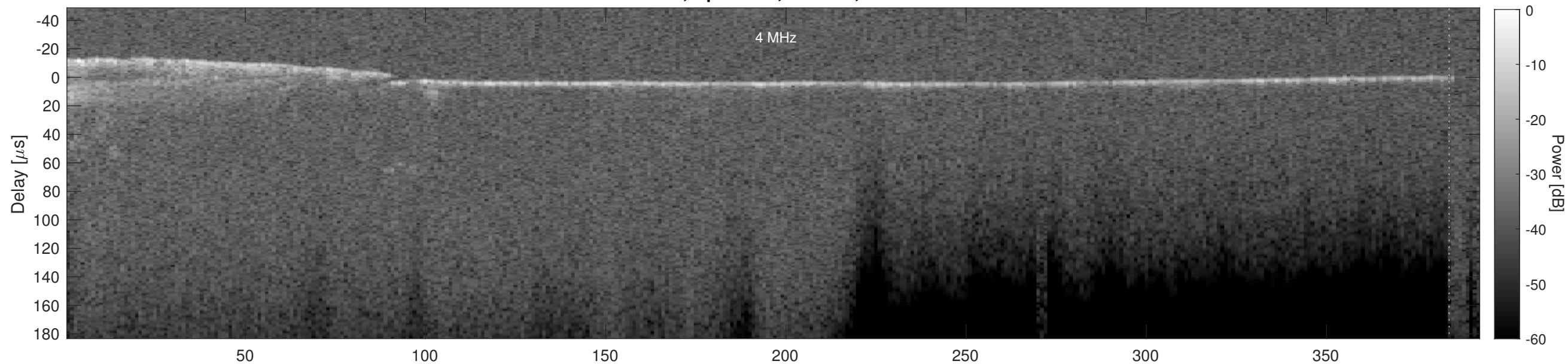
Orbit 5329, Cluttergram
