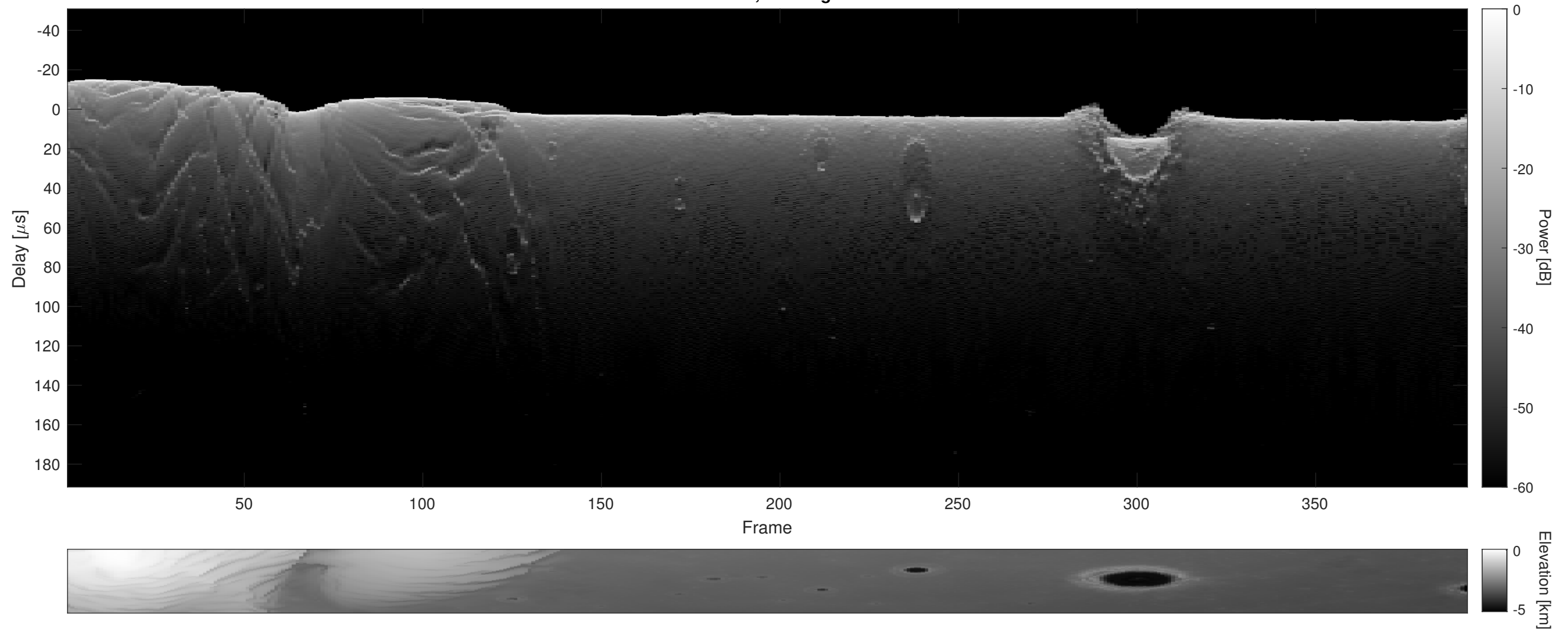
Orbit 5332, Cluttergram
