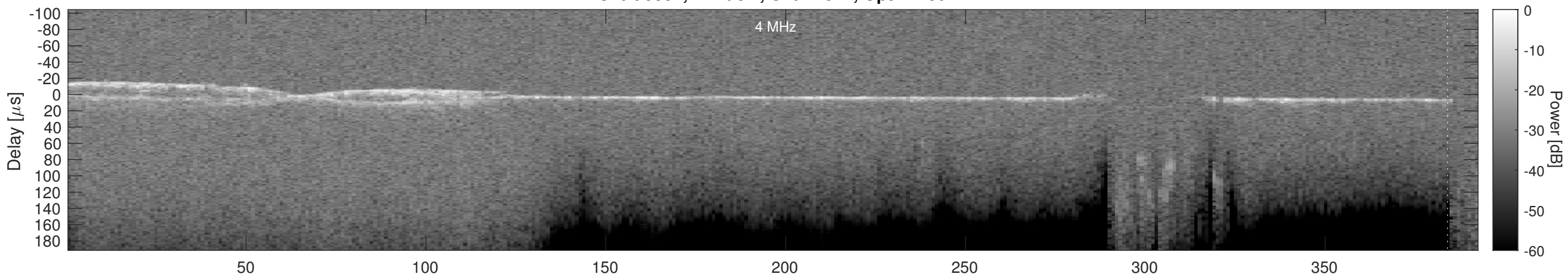
Orbit 5332, Cluttergram
