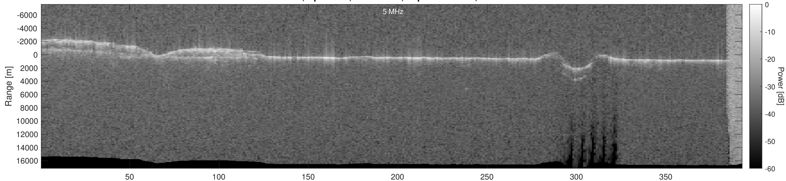
Orbit 5332, Optimized, No Window, Depth-Corrected, Channel 2
