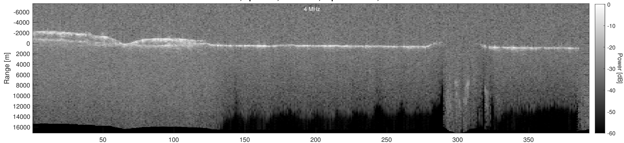
Orbit 5332, Depth-Corrected Cluttergram
