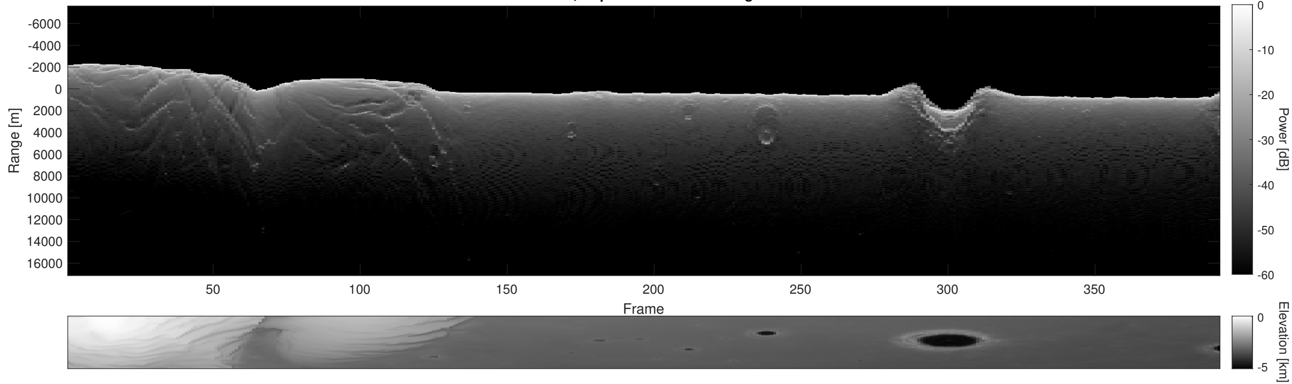
Orbit 5332, Depth-Corrected Cluttergram
