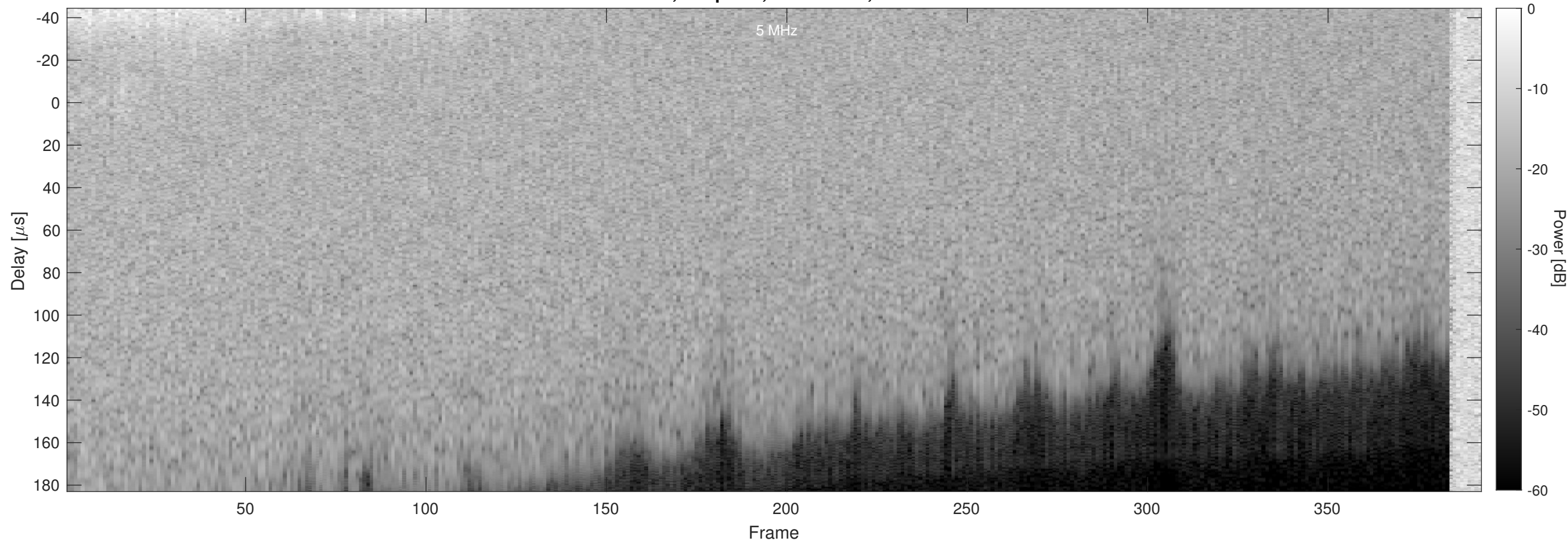
Orbit 5335, Chapman, No Window, Channel 2
