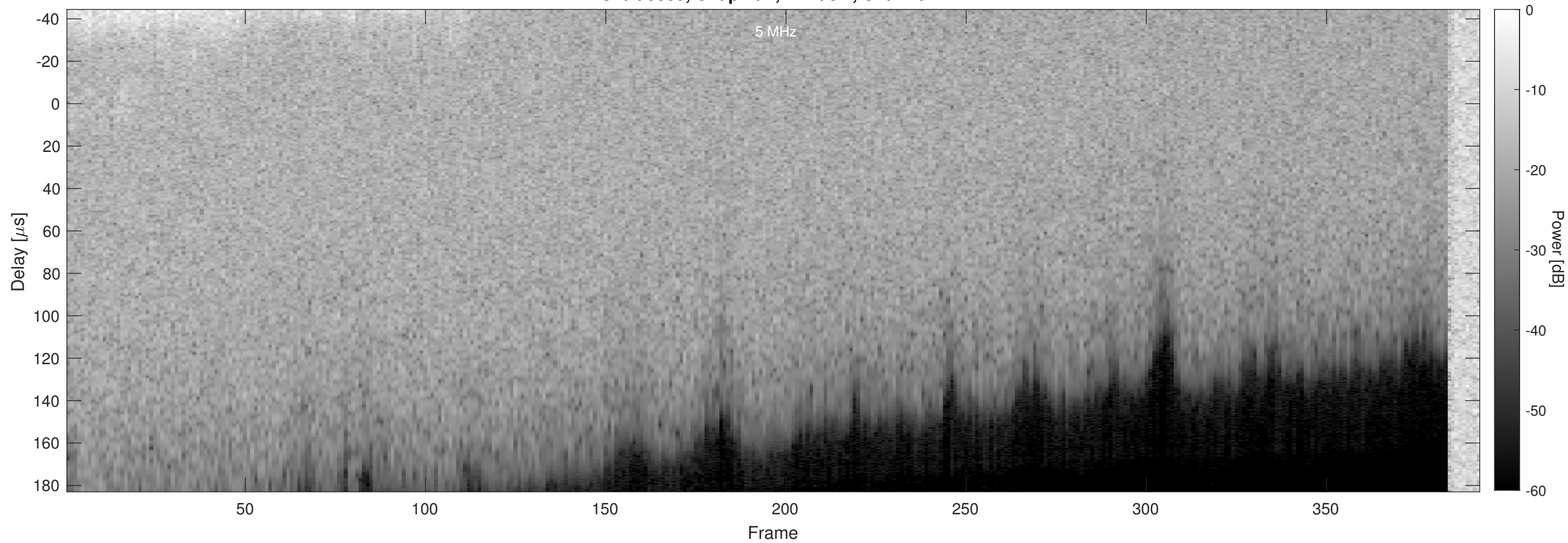
Orbit 5335, Chapman, Window, Channel 2
