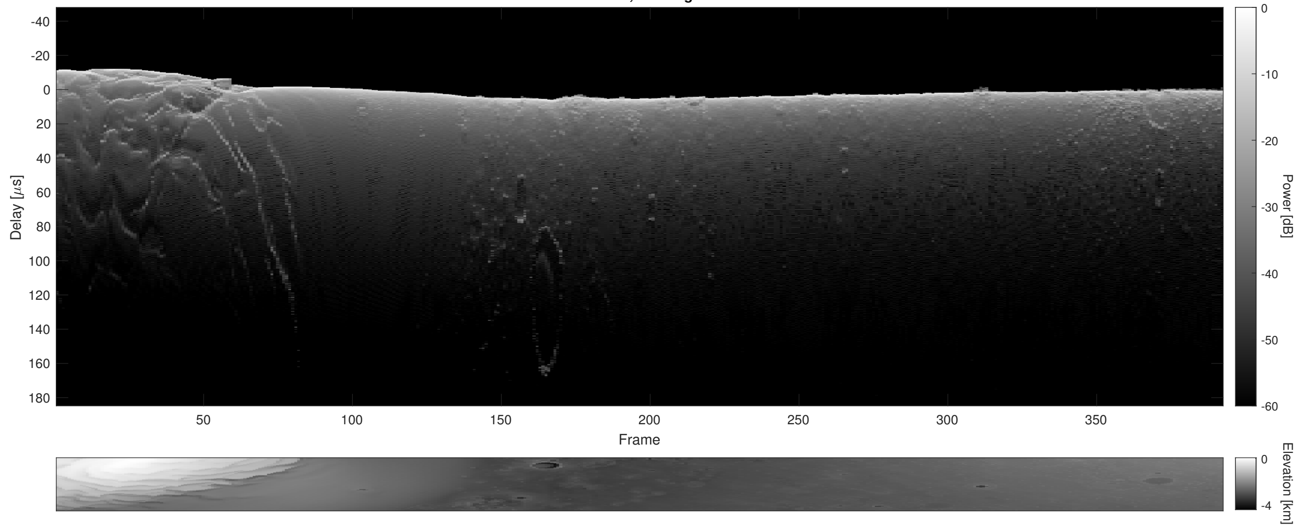
Orbit 5337, Cluttergram
