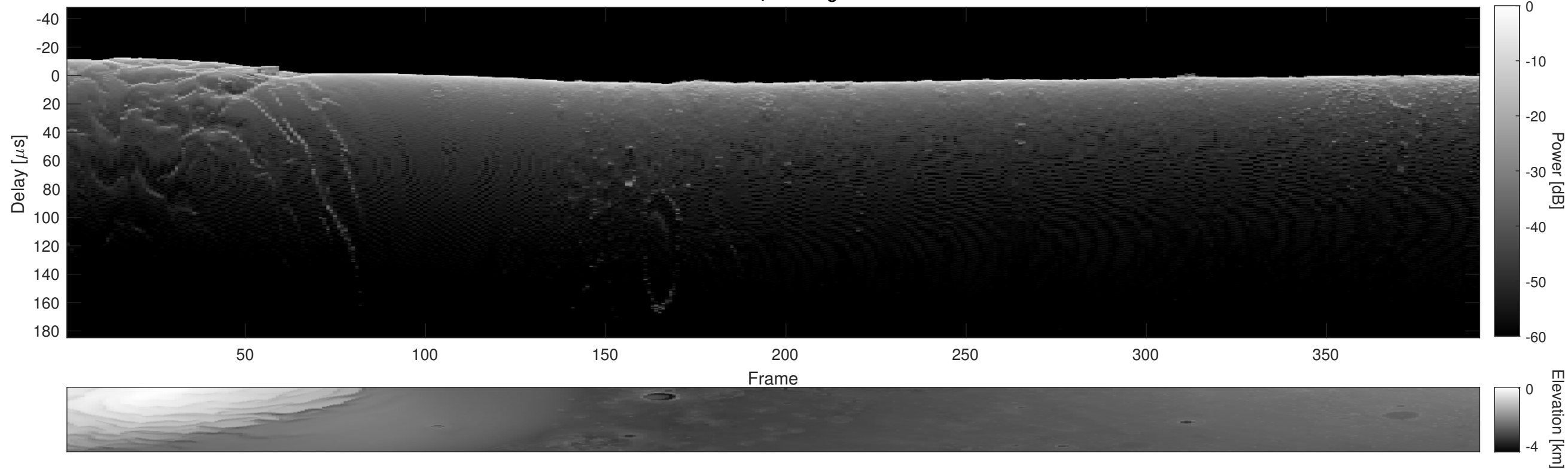
Orbit 5337, Cluttergram
