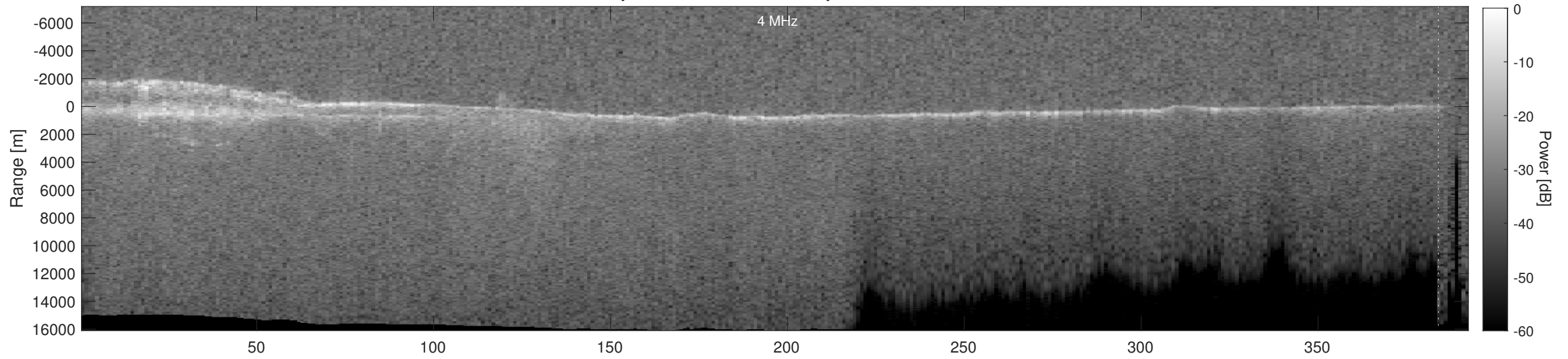
Orbit 5337, Depth-Corrected Cluttergram
