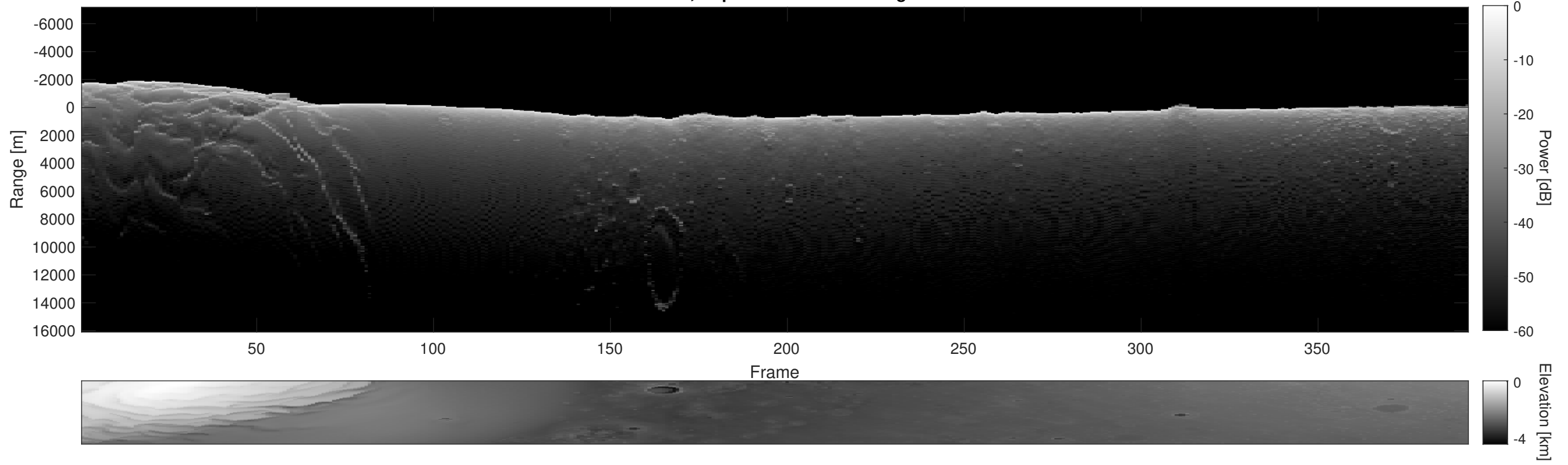
Orbit 5337, Depth-Corrected Cluttergram
