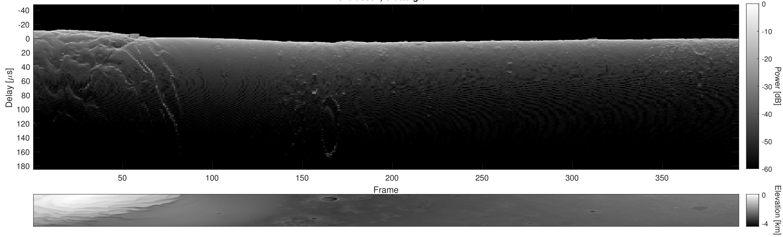
Orbit 5337, Cluttergram
