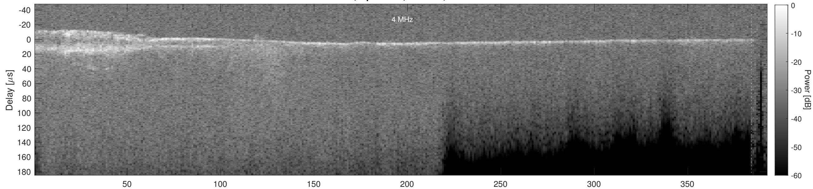
Orbit 5337, Cluttergram
