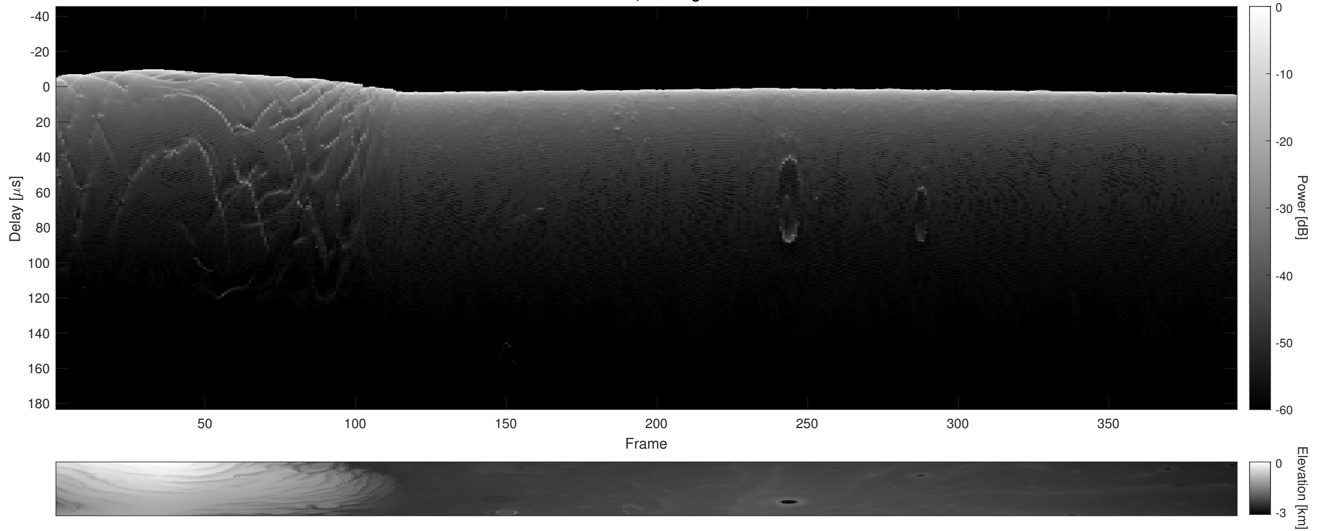
Orbit 5338, Cluttergram
