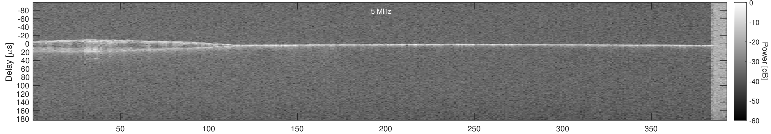
Orbit 5338, Cluttergram
