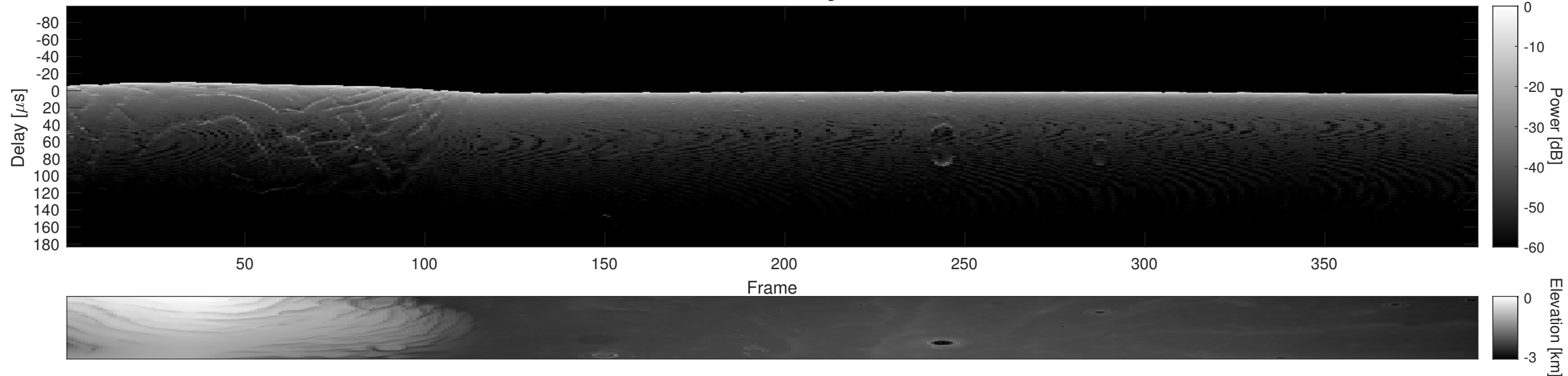
Orbit 5338, Cluttergram
