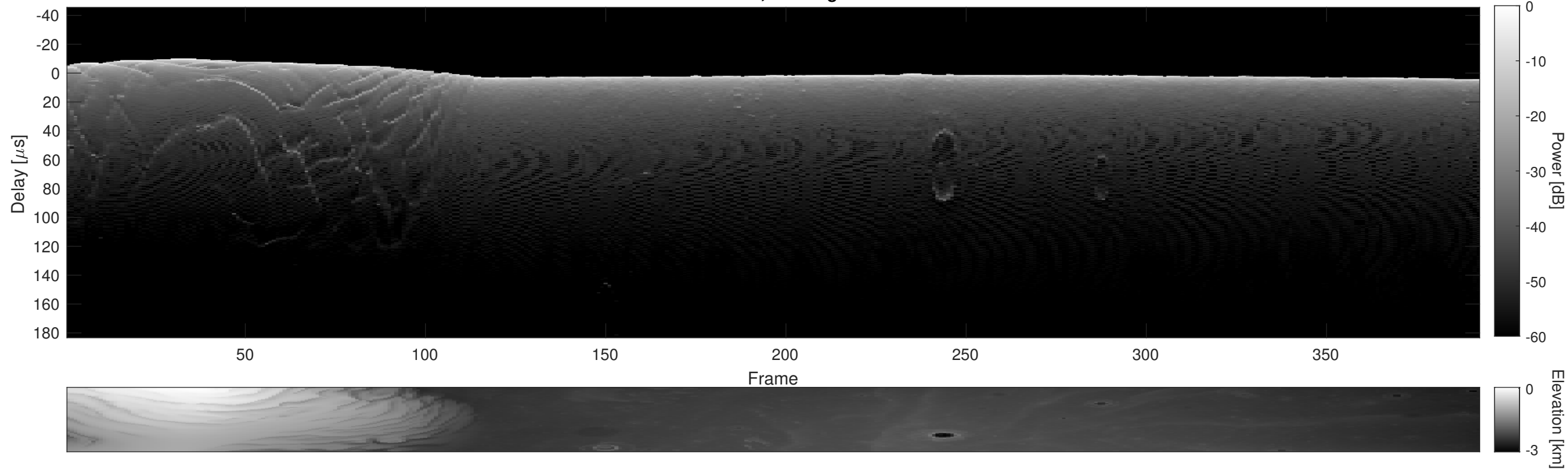
Orbit 5338, Cluttergram
