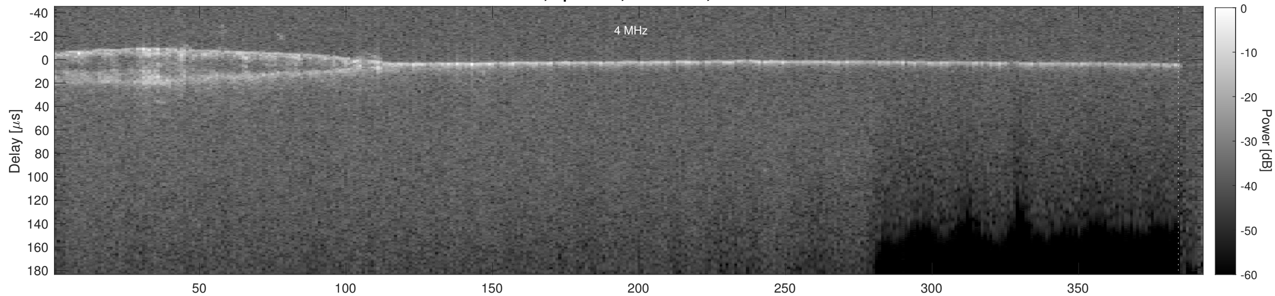
Orbit 5338, Cluttergram
