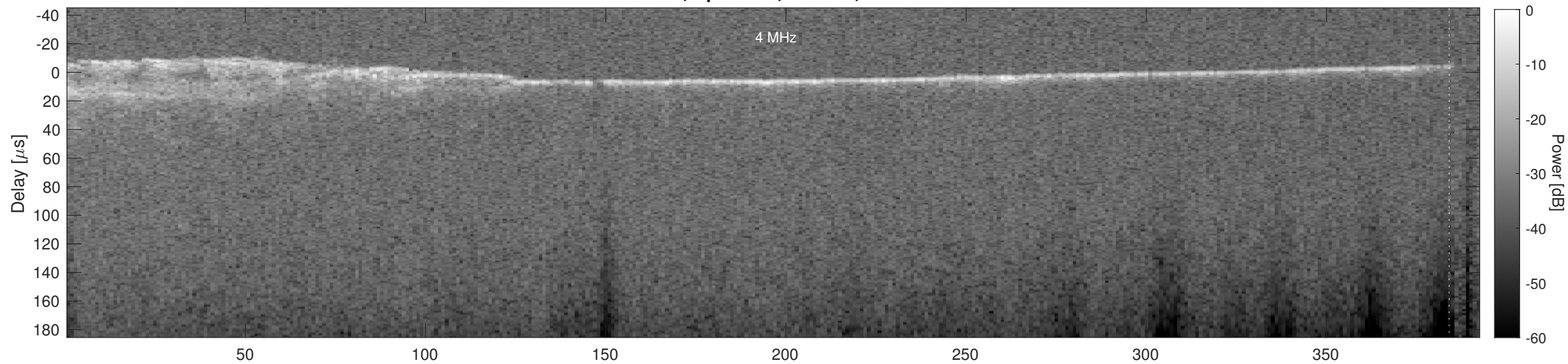
Orbit 5340, Cluttergram
