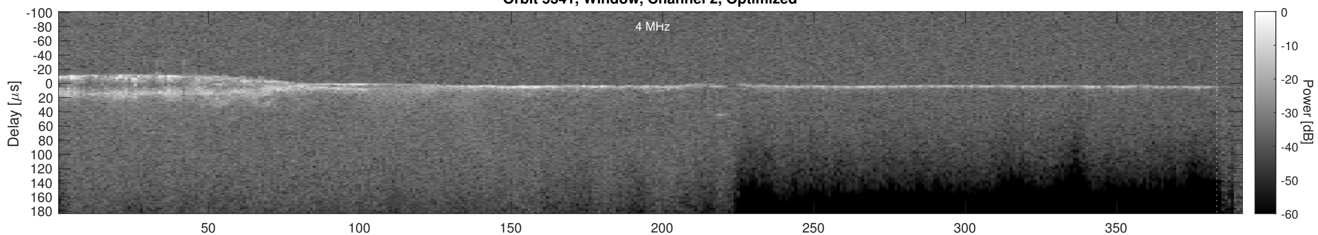
Orbit 5341, Cluttergram
