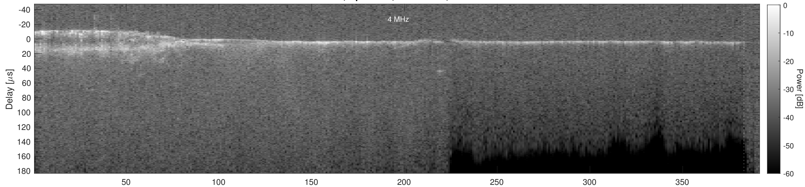
Orbit 5341, Cluttergram
