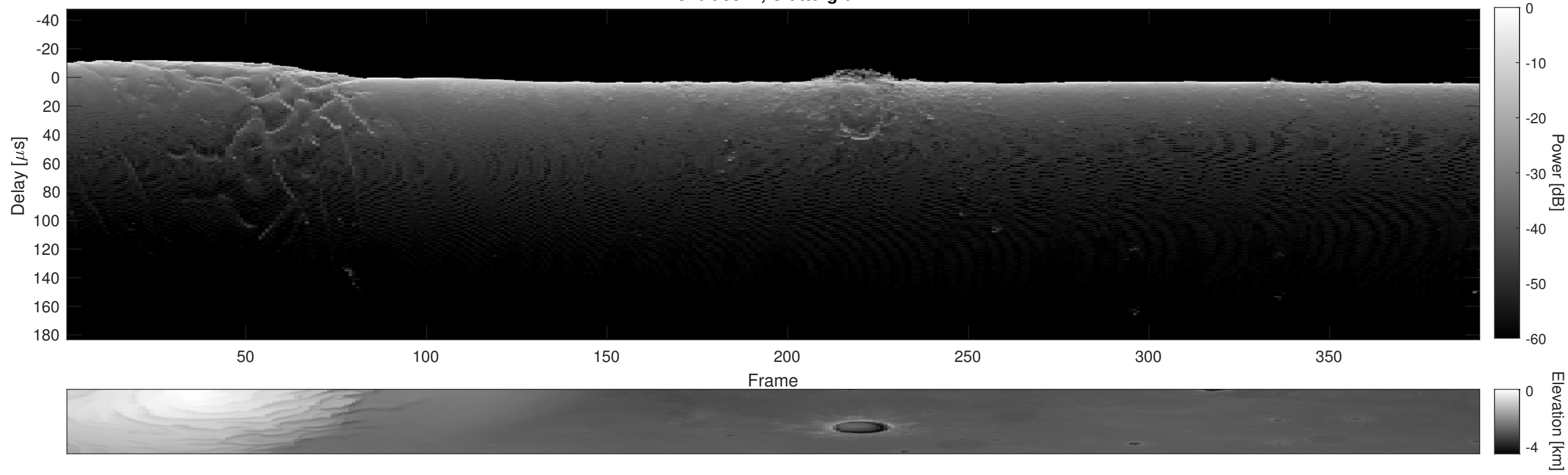
Orbit 5341, Cluttergram
