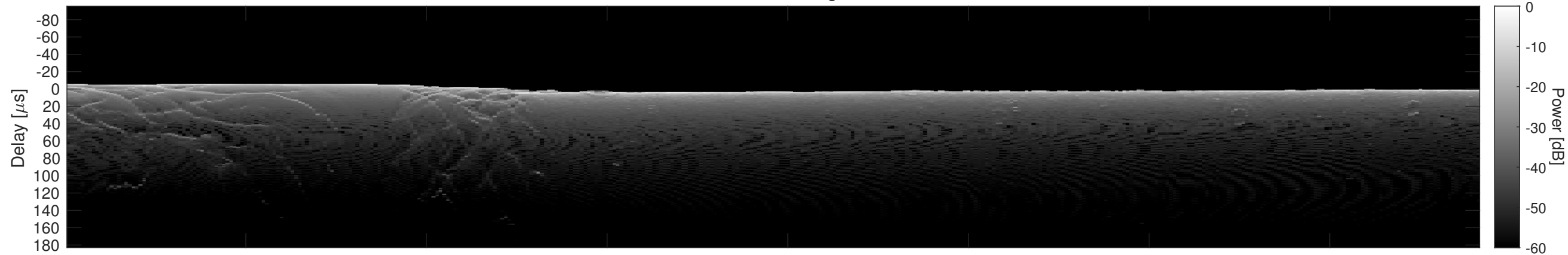
Orbit 5342, Cluttergram
