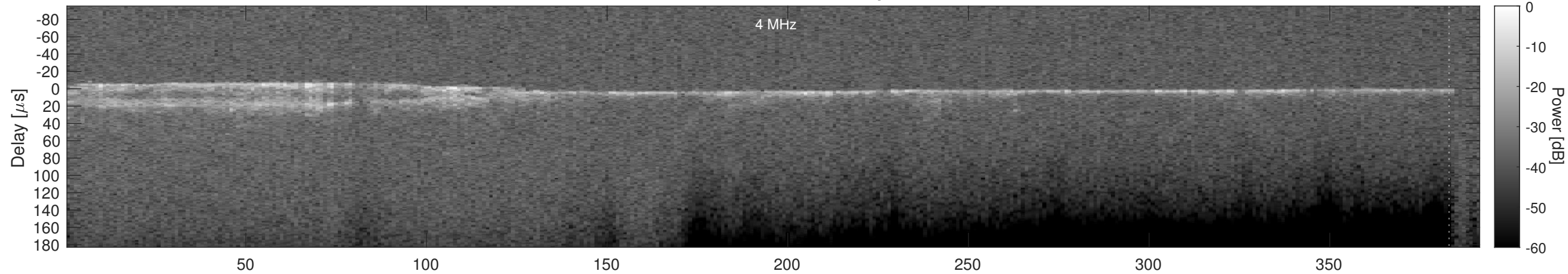
Orbit 5342, Cluttergram
